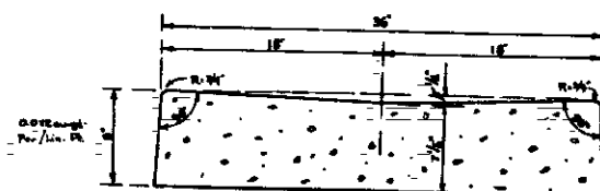
TYPICAL SECTION - P.C.C. CROSS GUTTER
