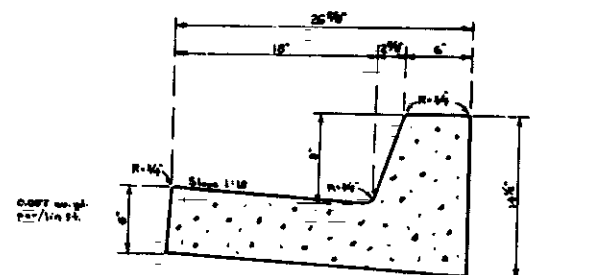
TYPICAL SECTION - P.C.C. CURB & GUTTER
