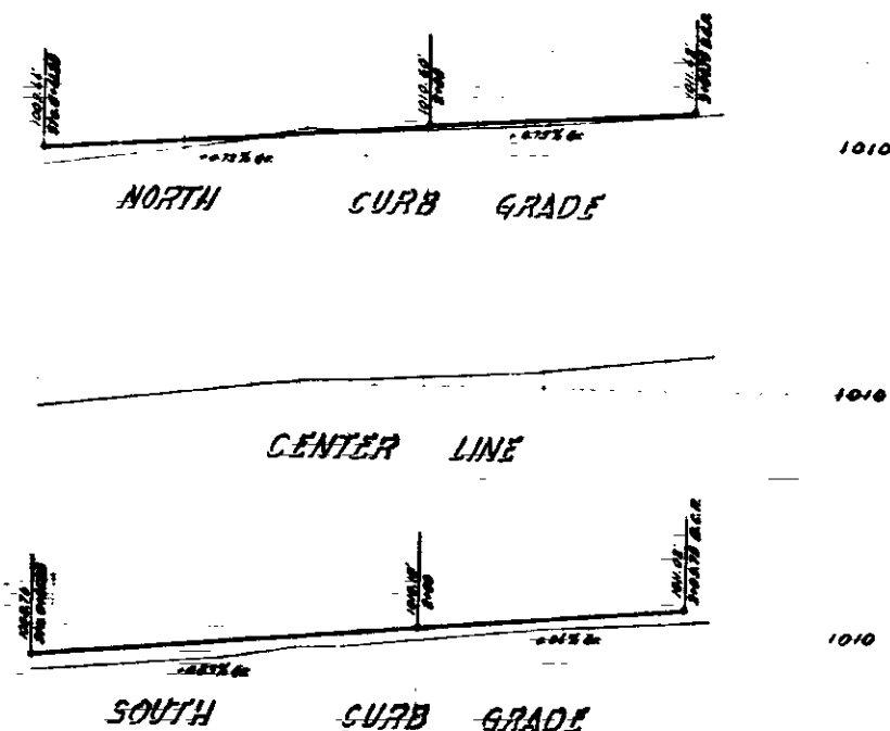
PROFILE REDICK STREET Scale: Horiz. 1"=40' Vert. 1"=4'
